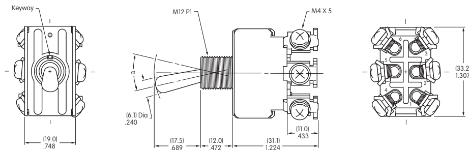
S421T does not have terminals 2 & 5
